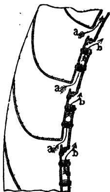
Ventilating Buckets.
